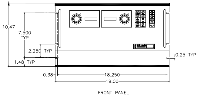
FRONT PANEL
