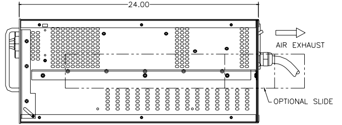
EXTENDED CHASSIS
