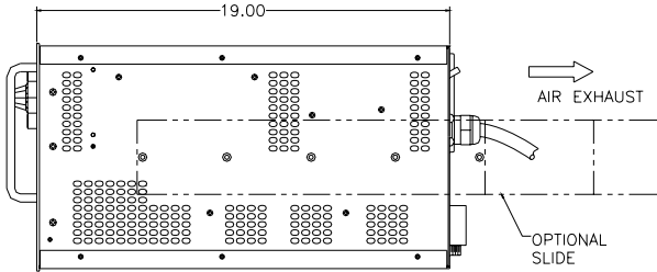
STANDARD CHASSIS
