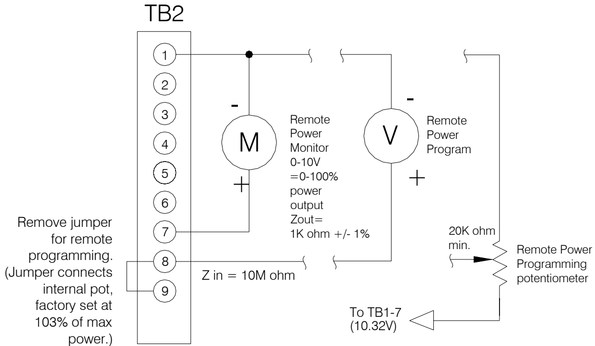
Figure 5.4 Adjustable Power Remote Interface
